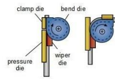
Rotary draw bending
