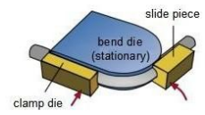
Compression bending
