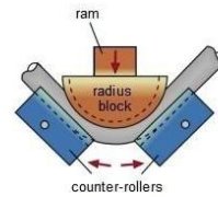
Ram bending
