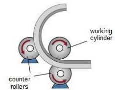
3 roll bending
